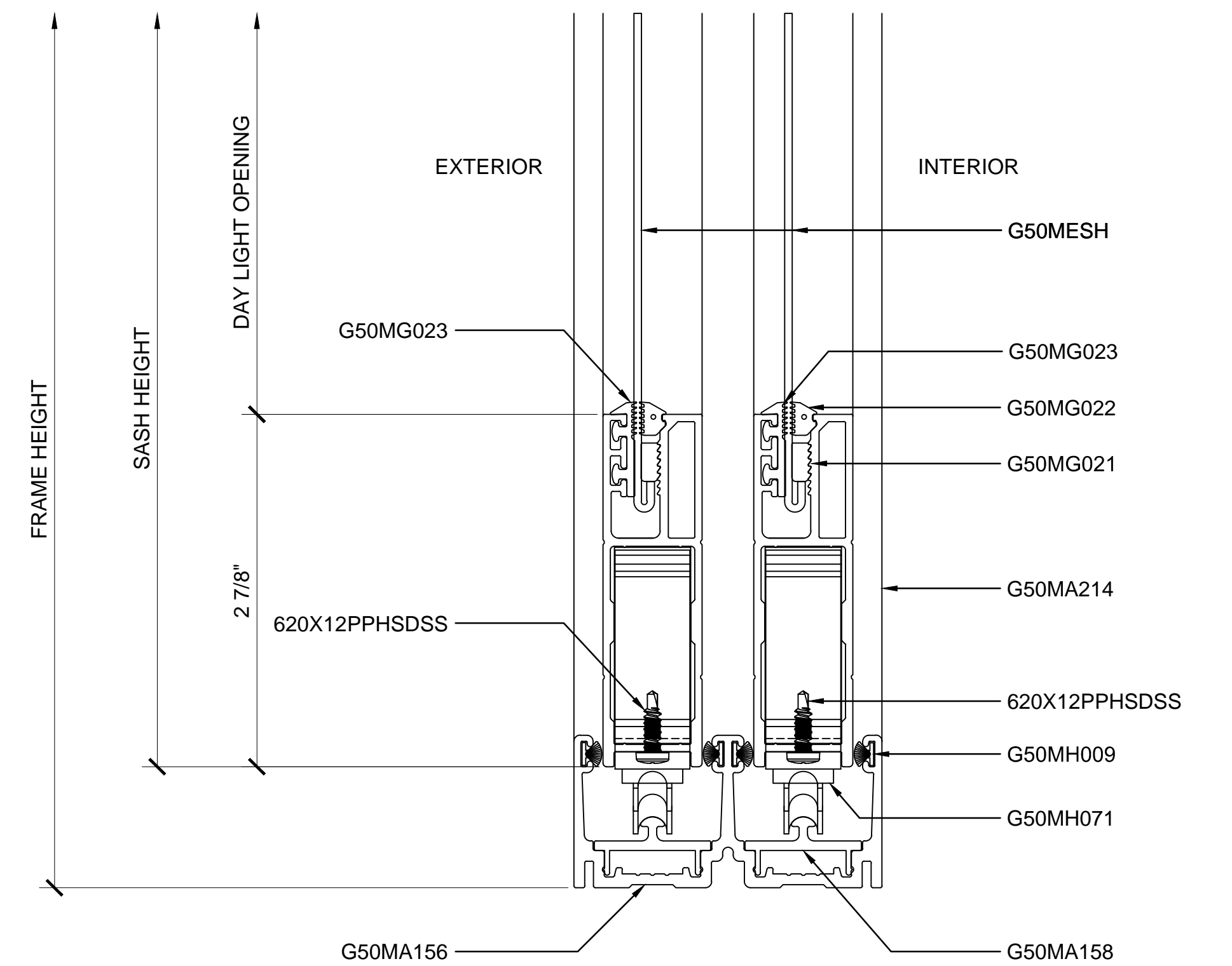
② SECTION DETAIL AT SILL ARCH REF: N/A 1'-0"=1'-0"
