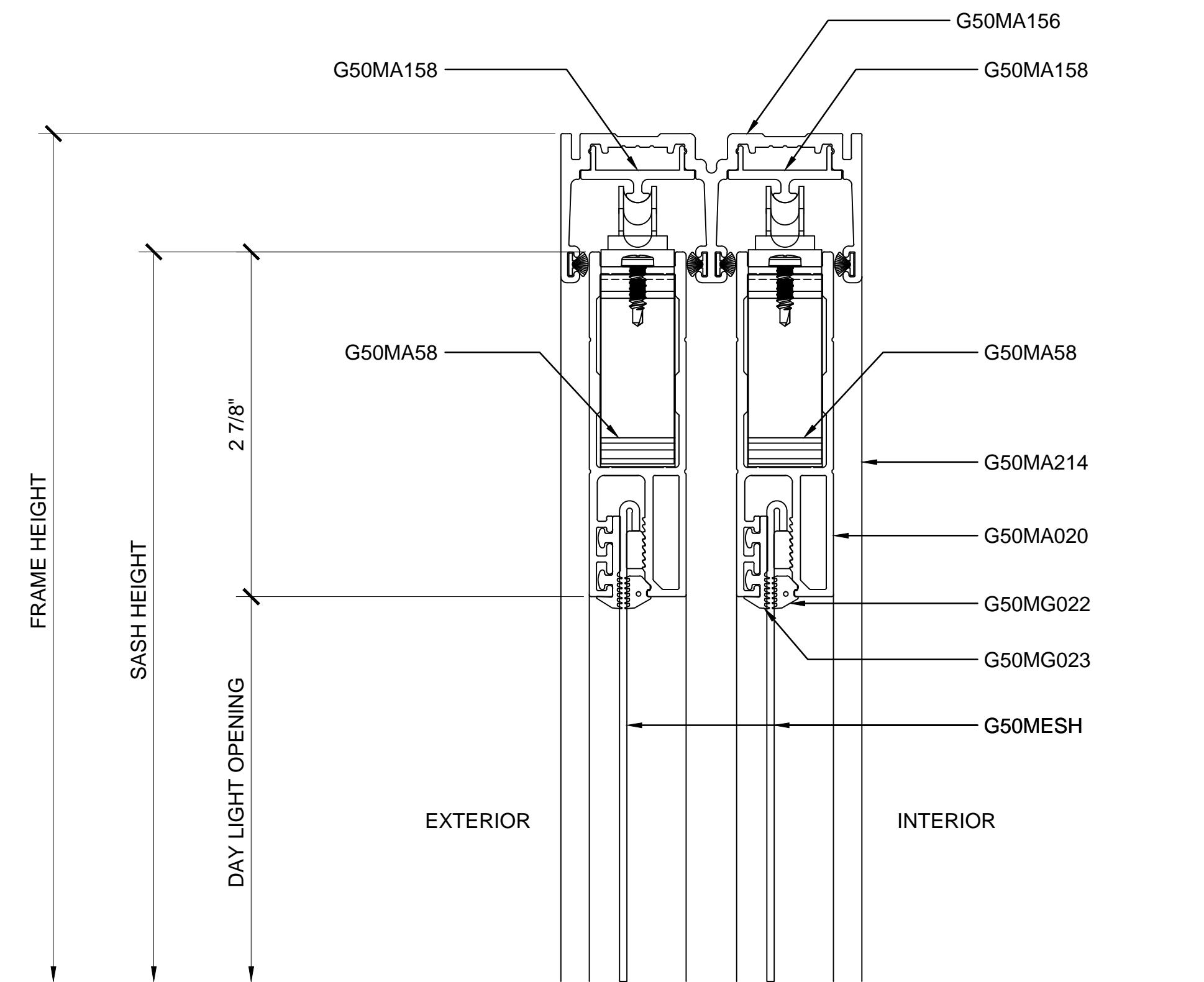
① SECTION DETAIL AT HEAD ARCH REF: N/A 1'-0"=1'-0"
